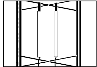
For backlit graphics, suspend fluorescent light from back scissor above the quad.
