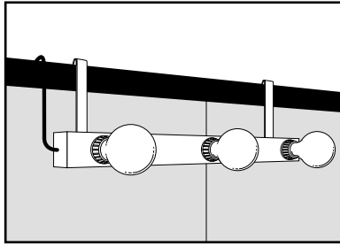
Center light bars. Drape cords behind display. Plug light cords into ElectroStrut power outlet strip at the back of the frame.
