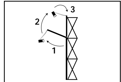
Rotate top section of strut up and slide down onto top stud.
