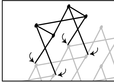
Place frame in position. Slide hook ends of frame into slots located in front and back hubs.
