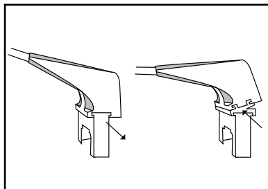
For low ceiling environments, remove sleeve connector and replace with Low Ceiling Mounting Clip.
