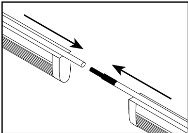
Connect fluorescent light fixtures by joining sections.
