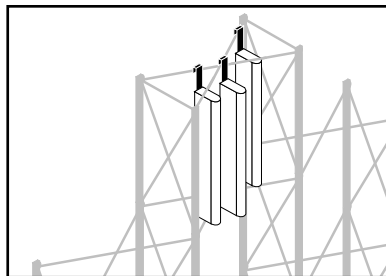
Hang optional fluorescent lights from back scissor of frame.
