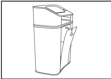
FabriCounter/Lectern Fabric Door (optional accessory). Insert door into groove of bottom shelf with pull-tab outward. Flex door and tuck it into groove along the underside of middle shelf. To open door, simply pull downward on tab.
