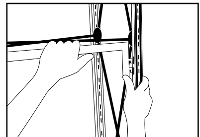
Insert the mid-level bridge brace securely into the side of the connected struts.
