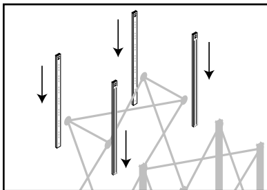
Slide extended quad struts onto all four sides.
