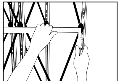
Insert the mid-level bridge brace securely into the connected struts.
