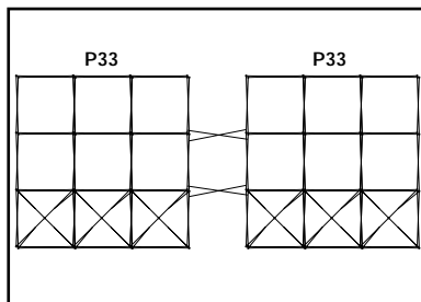
Place frames side-by-side and unfold connecting scissors carefully.
