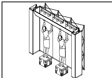
Hang the Plus HeadLiner frame by the brackets. We recommend that two people lift and hang the HeadLiner.
