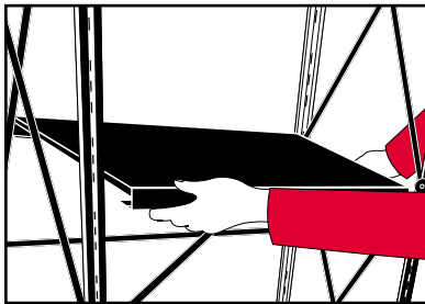
Press shelf down onto frame scissor. Maximum shelf load is 50 lbs / 23 kg; heavier load may cause failure.
