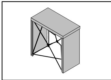
Press DemiTable top shelf down onto frame scissors, ensuring that snap clips are engaged. NOTE: Maximum load is 50 lbs / 23 kgs; heavier load may cause failure.
