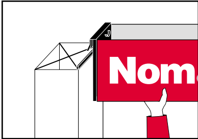
Hook bridge onto bridge braces between two displays or a display and column.
