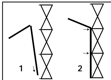
Slide bottom of connected strut onto the stud at the bottom of the frame. Snap next two connectors onto studs on frame.
