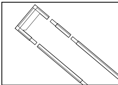
Lay end pieces opposite each other. Place segments in between, all ends should match up male to female.
