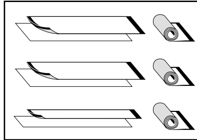
Roll individual Tempo fabric or Photomural Panels with liners in between and roll fabric/image side out. Repeat same for End Caps.
